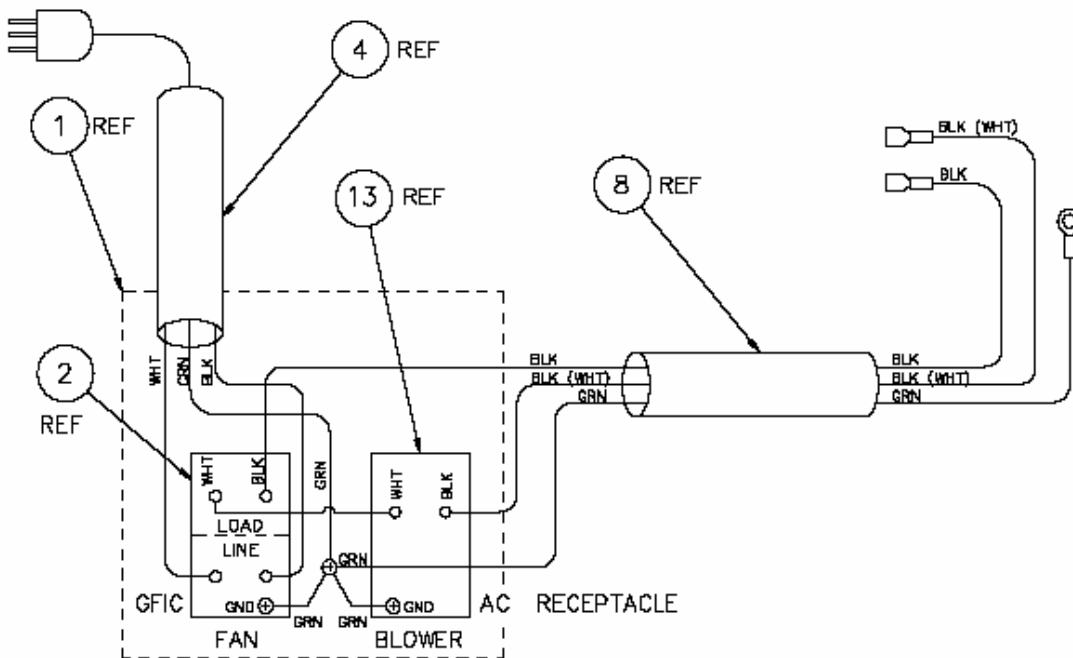
SIMPLIFIED WIRING DIAGRAM
